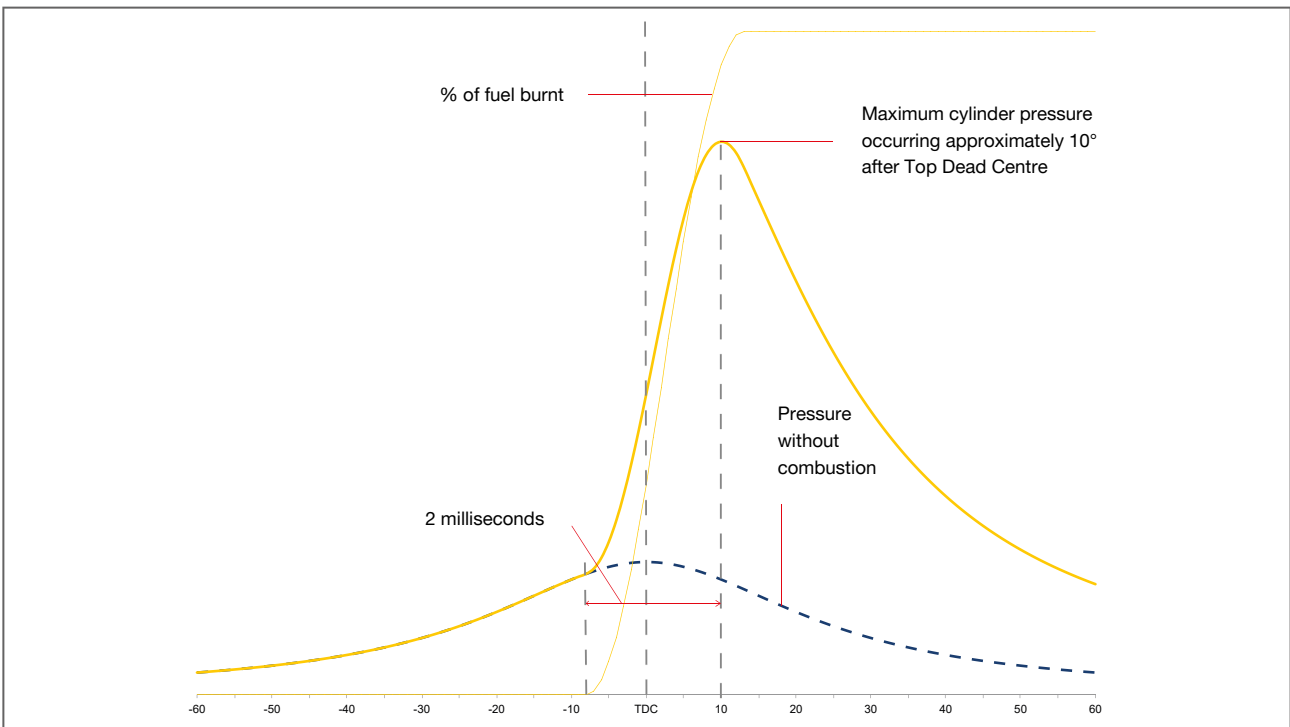
Fig 3.9 Setting ignition timing approximately 2 milliseconds before maximum cylinder pressure is required
