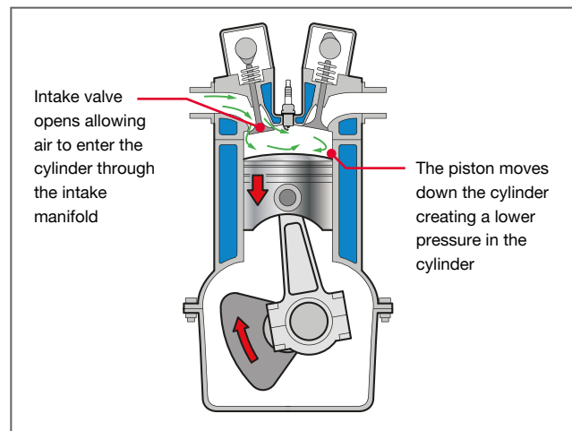
Fig 2.1 Intake stroke
