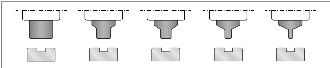
Fig 7.3 Examples of different types and sizes of centre electrodes
